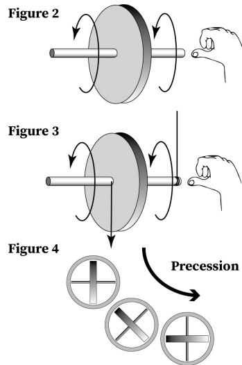
Figure 5.116 Direction of Angular Momentum
