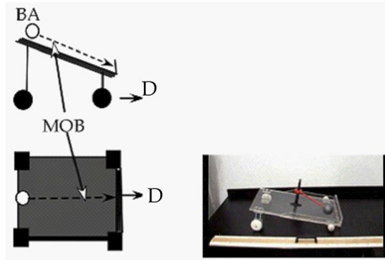
Figure 5.2 Kinetic Drive (KD) [Fair Use]
