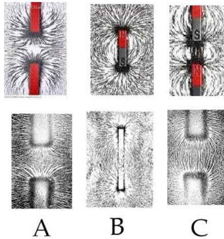
Figure 5.103 Comparing Magnetic Fields [Fair Use]
