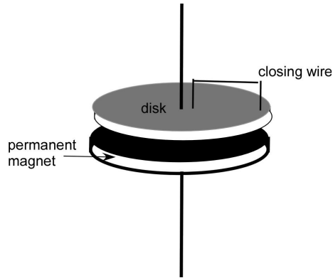
Figure 5.21 Schematic of the Homopolar Generator
