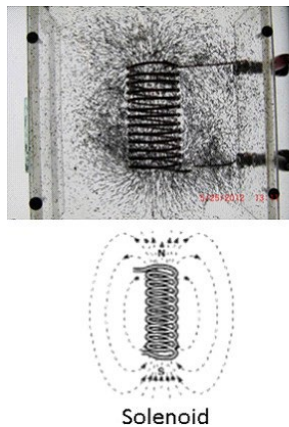
Solenoid
