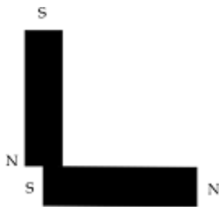
Figure 5.96 L-shaped PMs
