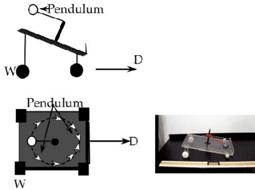
Figure 5.3 Pendulum Drive (PD) [Fair Use]
